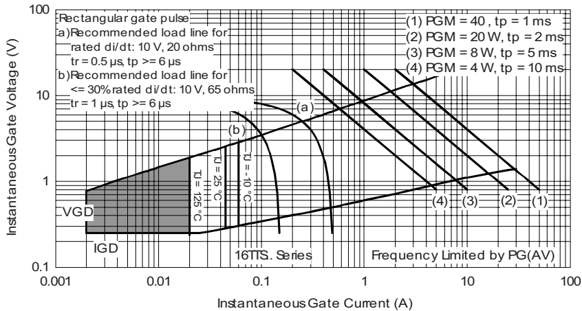
Fig. 9 - Gate Characteristics
